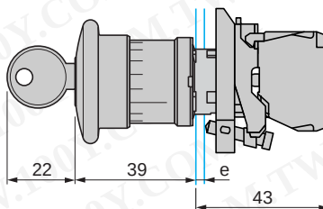
XB4-BS142, BS9445
