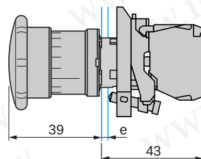
XB4-BS542, BS8445
